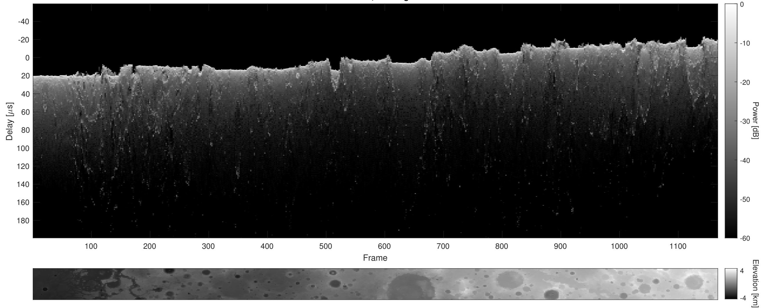
Orbit 15555, Cluttergram
