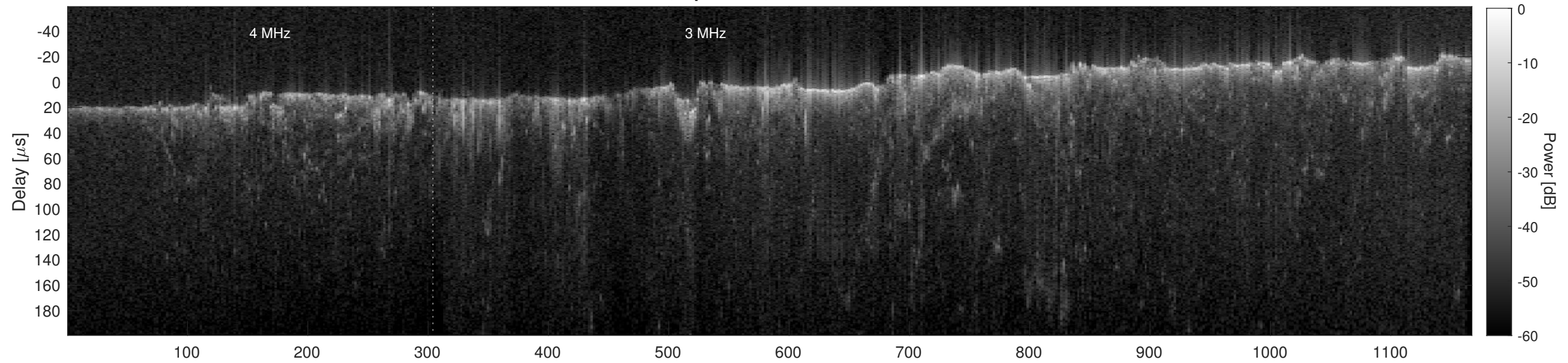
Orbit 15555, Cluttergram
