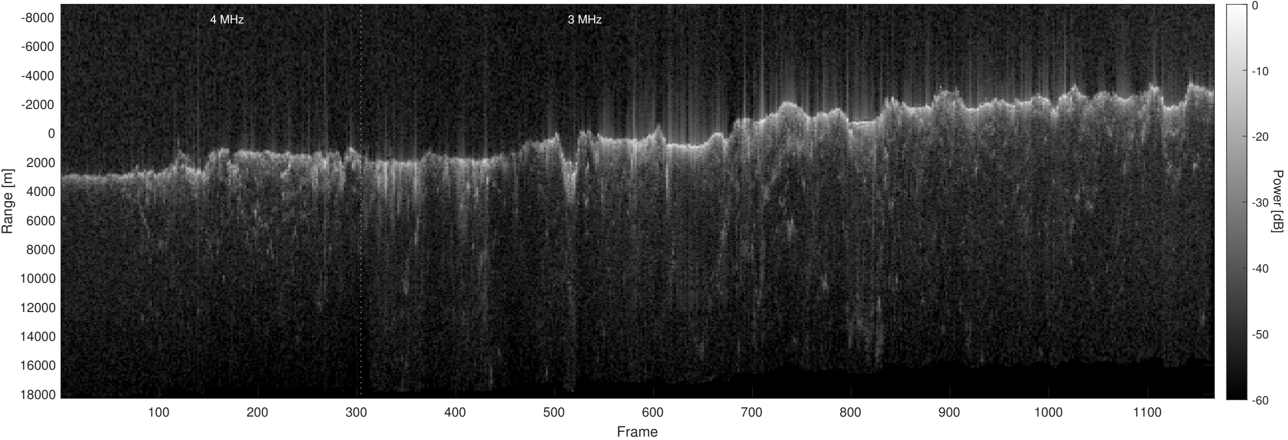
Orbit 15555, Optimized, No Window, Depth-Corrected, Channel 2
