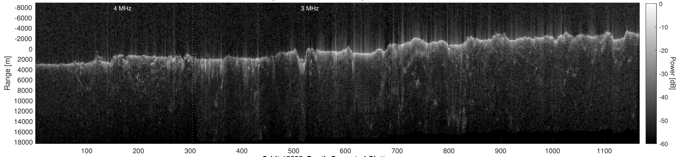
Orbit 15555, Depth-Corrected Cluttergram
