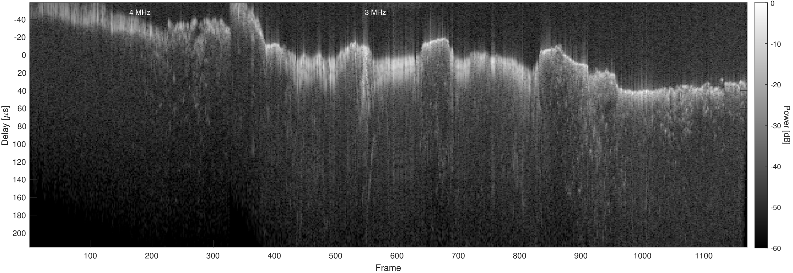
Orbit 15558, Chapman, No Window, Channel 2
