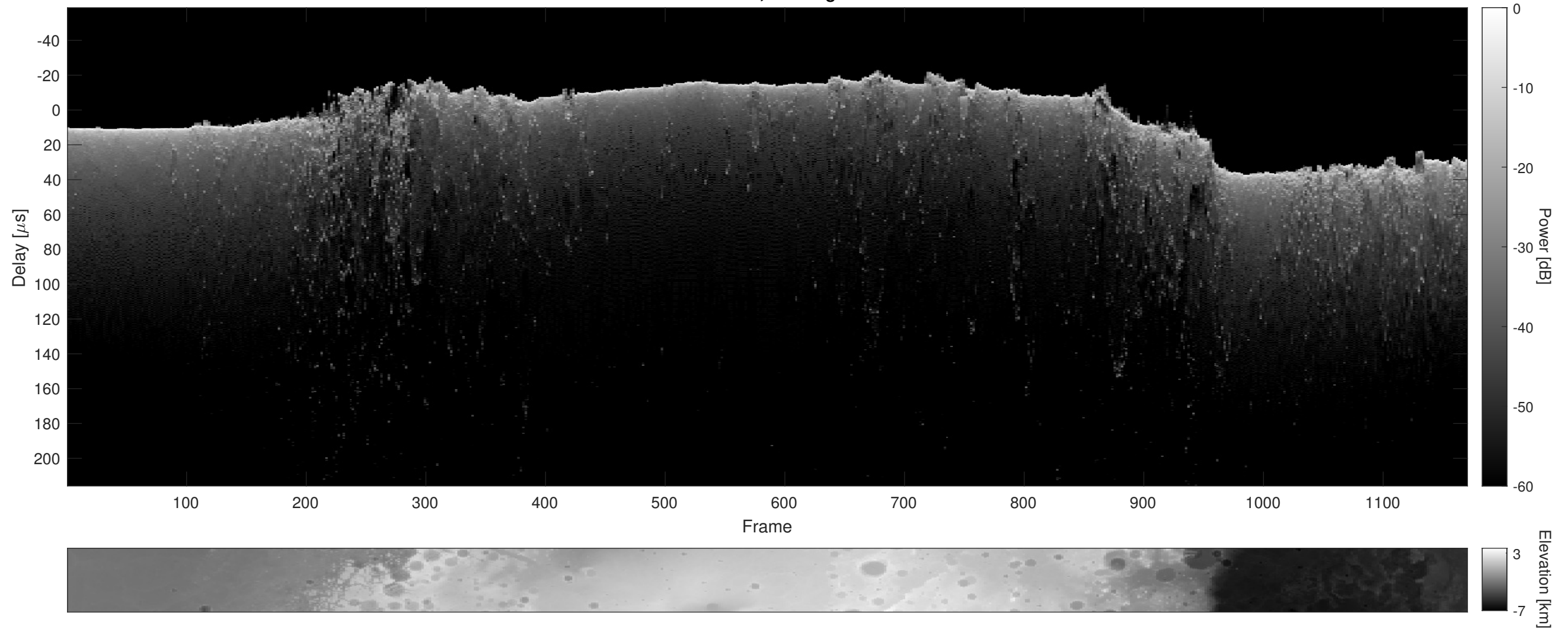
Orbit 15558, Cluttergram
