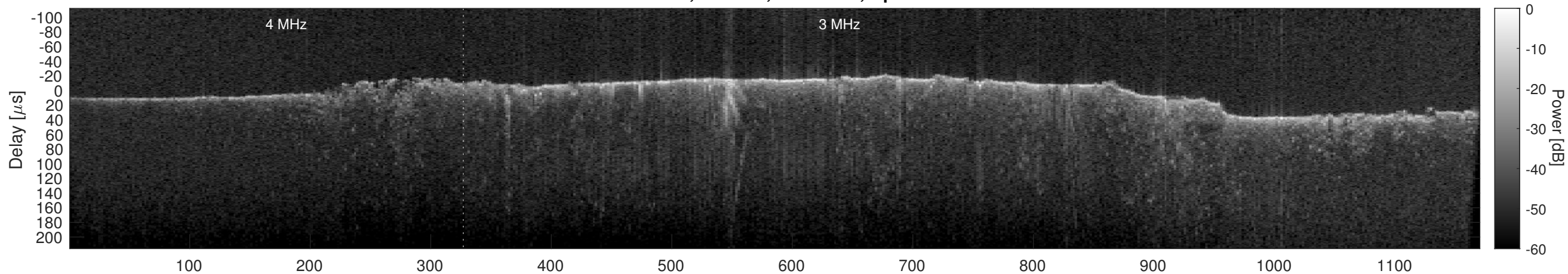
Orbit 15558, Cluttergram
