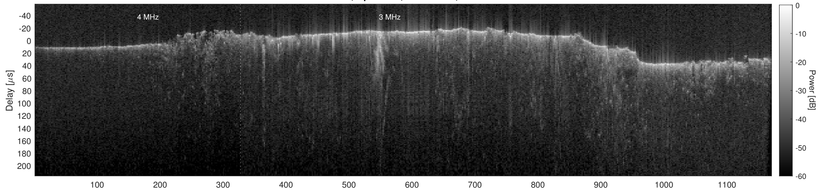
Orbit 15558, Cluttergram
