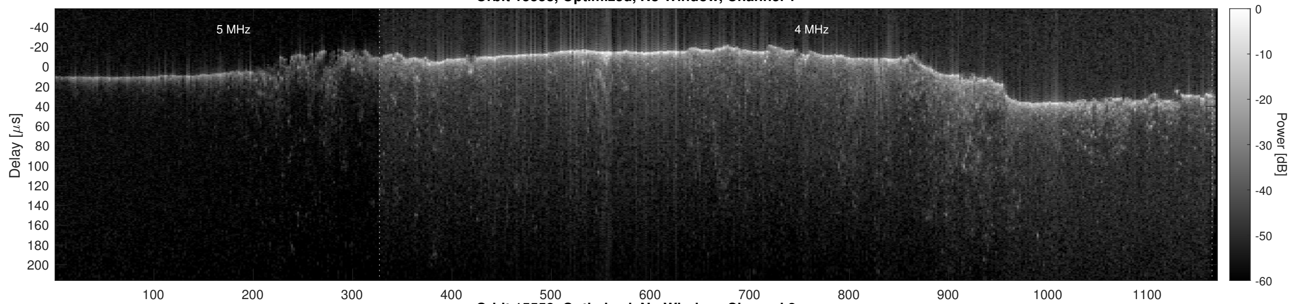
Orbit 15558, Optimized, No Window, Channel 2
