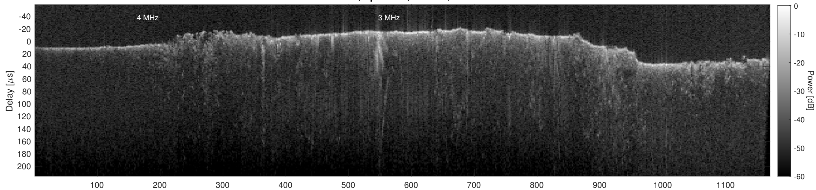
Orbit 15558, Cluttergram
