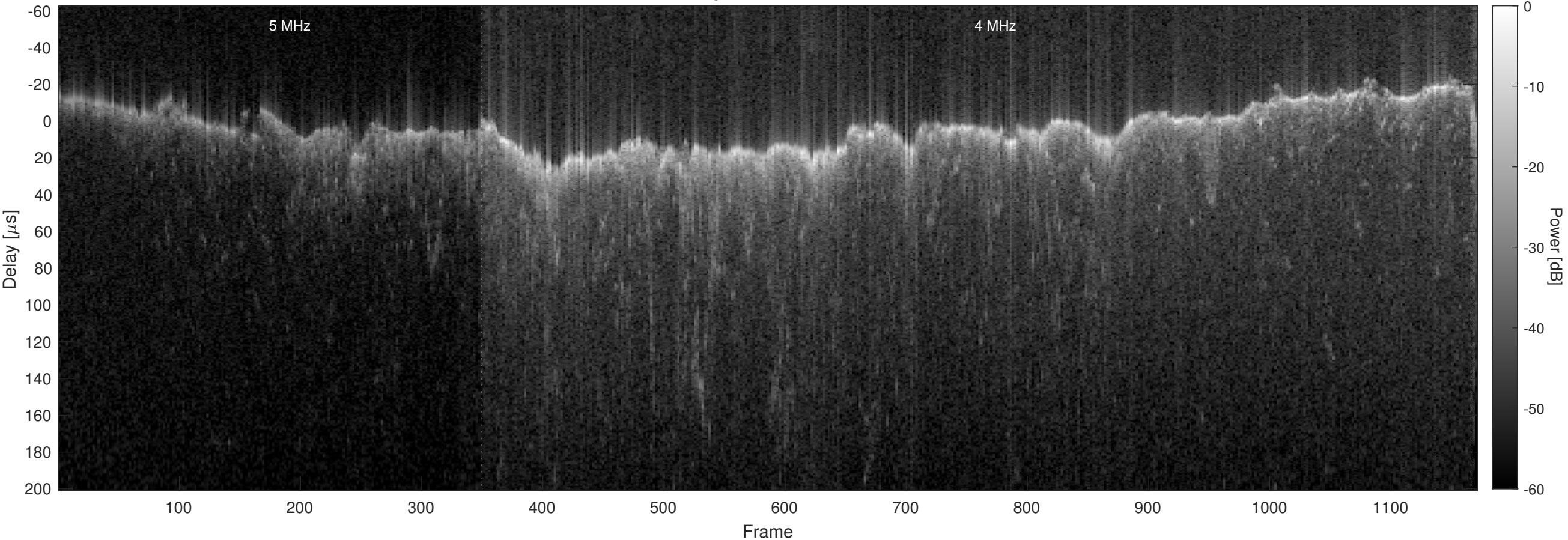
Orbit 15562, Chapman, No Window, Channel 2
