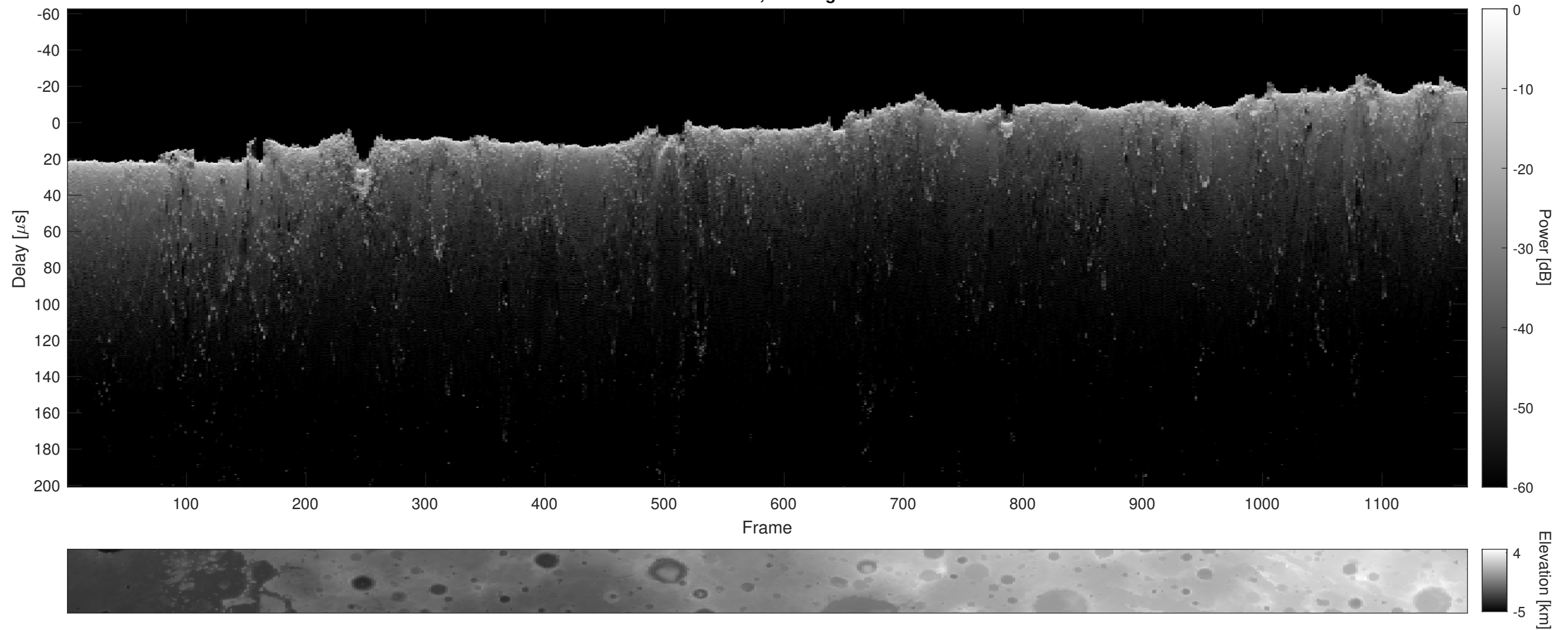
Orbit 15562, Cluttergram
