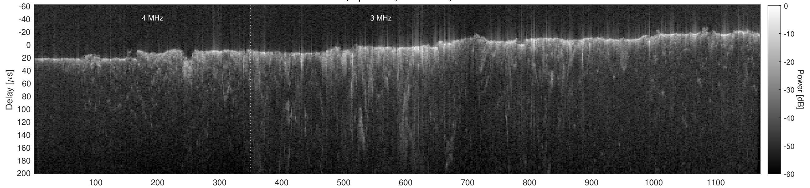
Orbit 15562, Cluttergram
