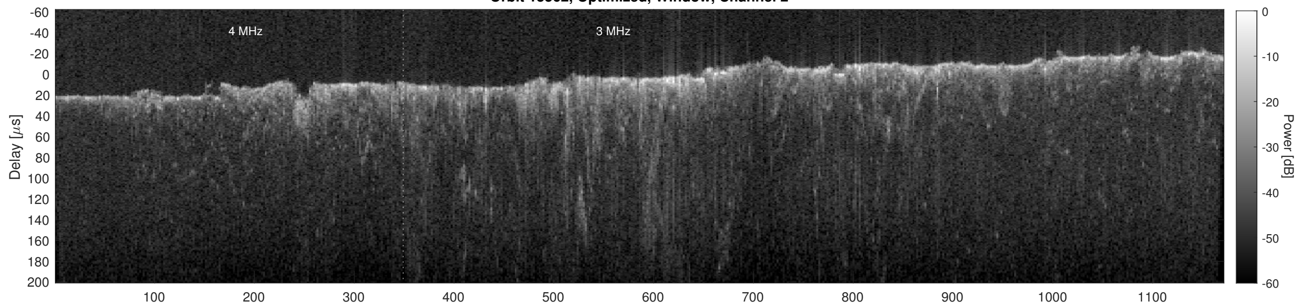
Orbit 15562, Cluttergram
