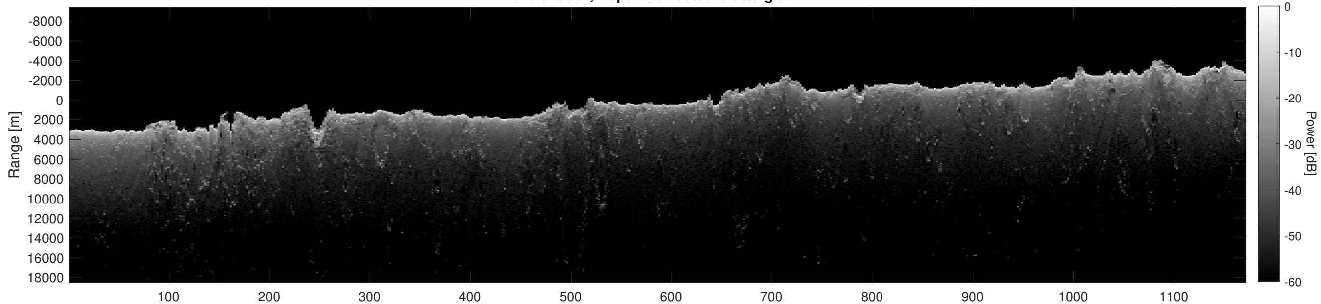
Orbit 15562, Depth-Corrected Cluttergram
