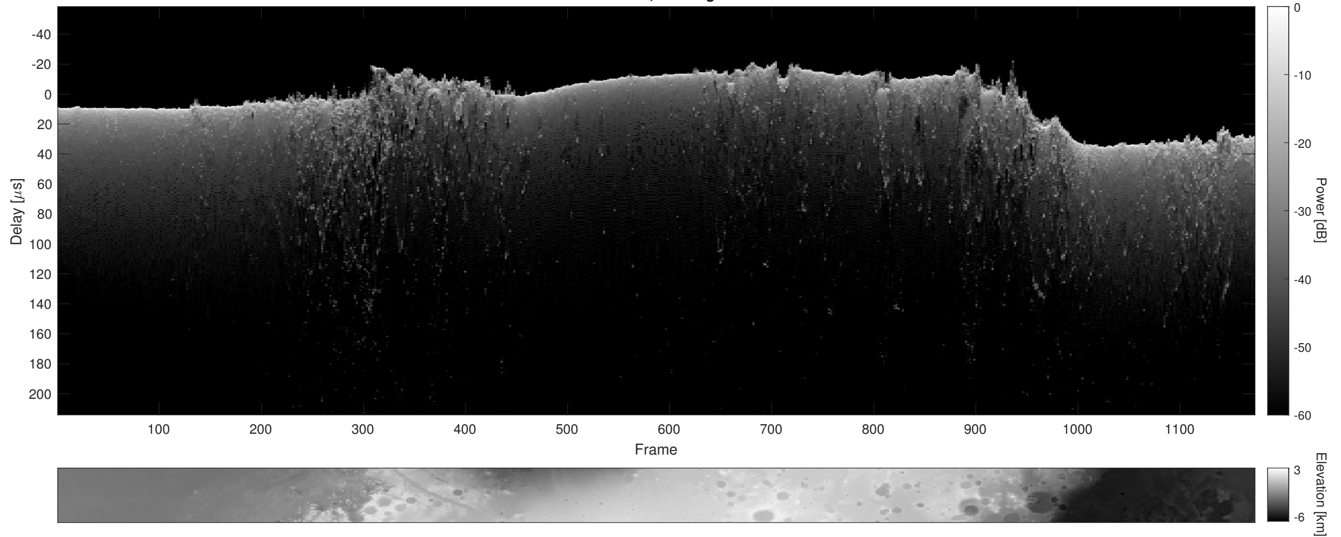
Orbit 15565, Cluttergram
