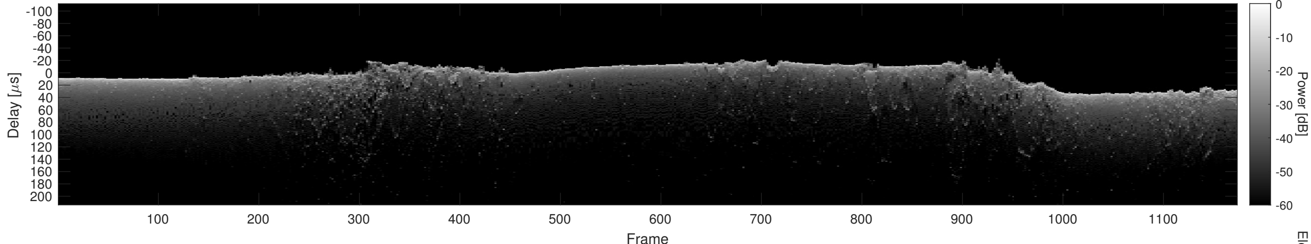
Orbit 15565, Cluttergram
