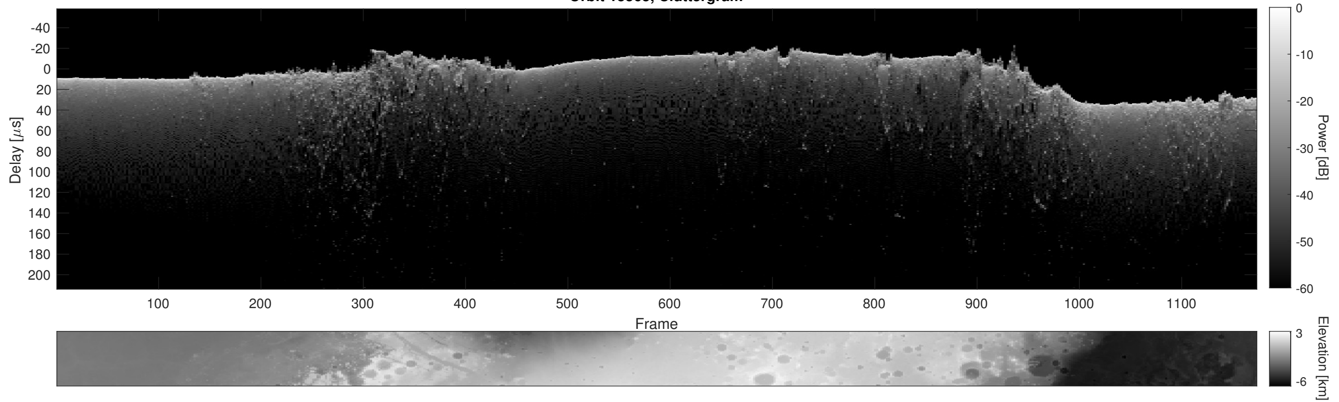
Orbit 15565, Cluttergram
