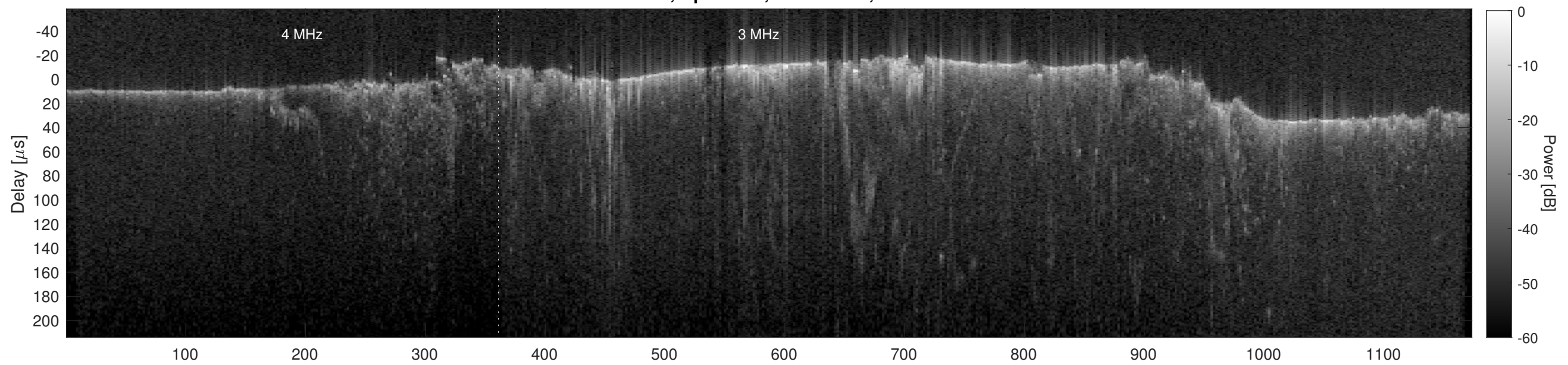
Orbit 15565, Cluttergram
