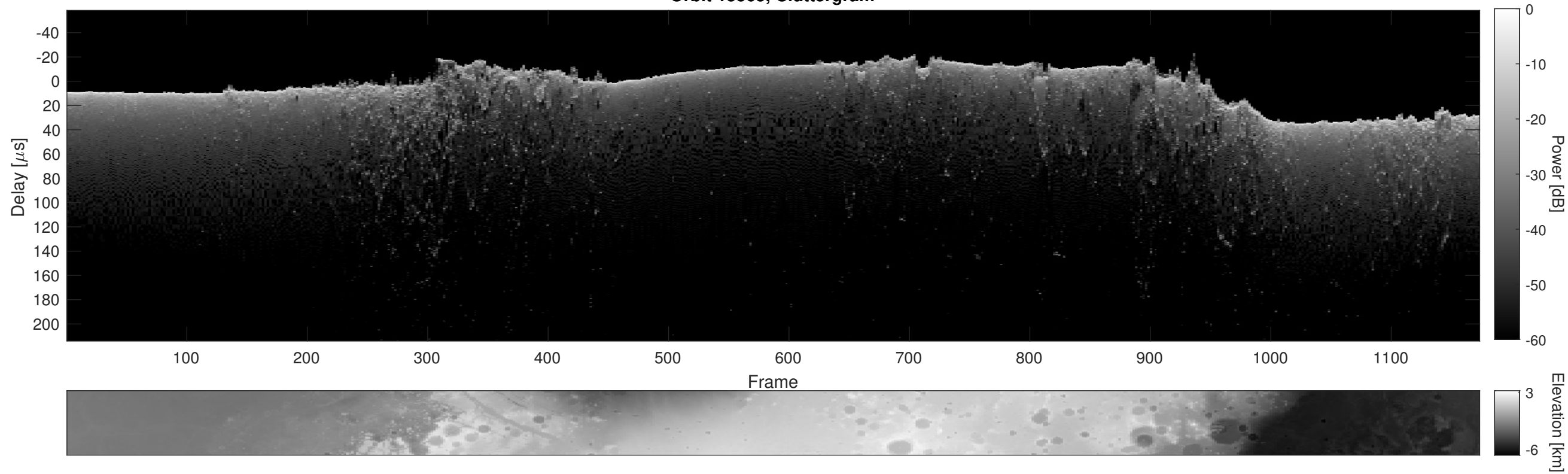
Orbit 15565, Cluttergram
