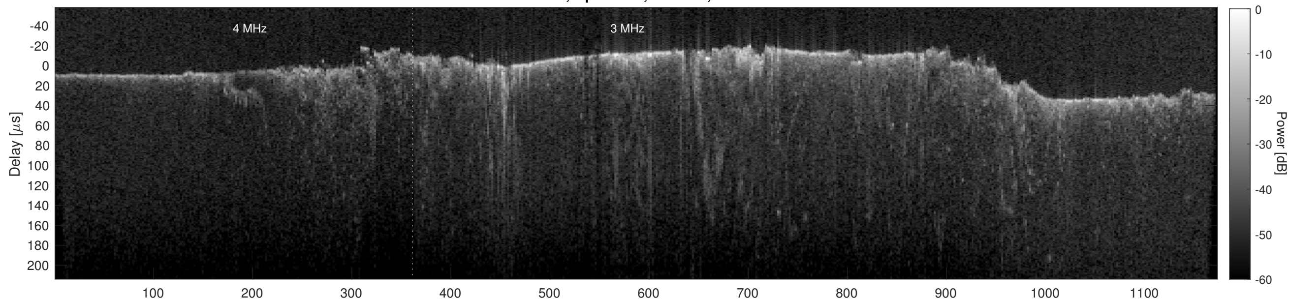
Orbit 15565, Cluttergram
