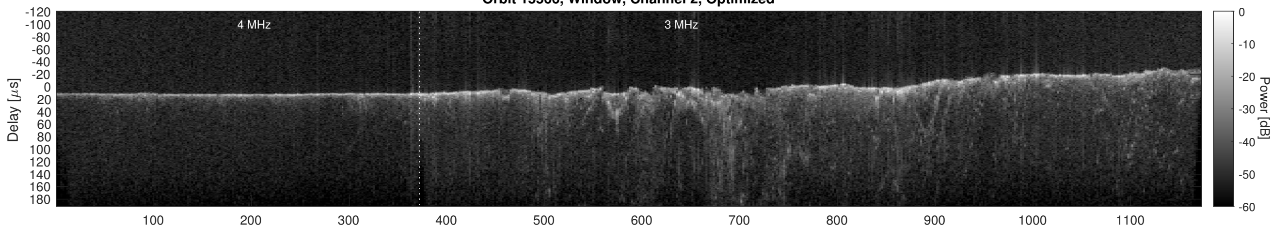
Orbit 15566, Cluttergram
