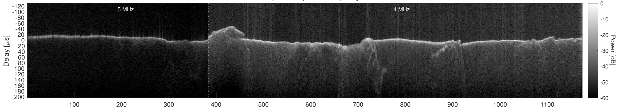
Orbit 15567, Window, Channel 1, Optimized
