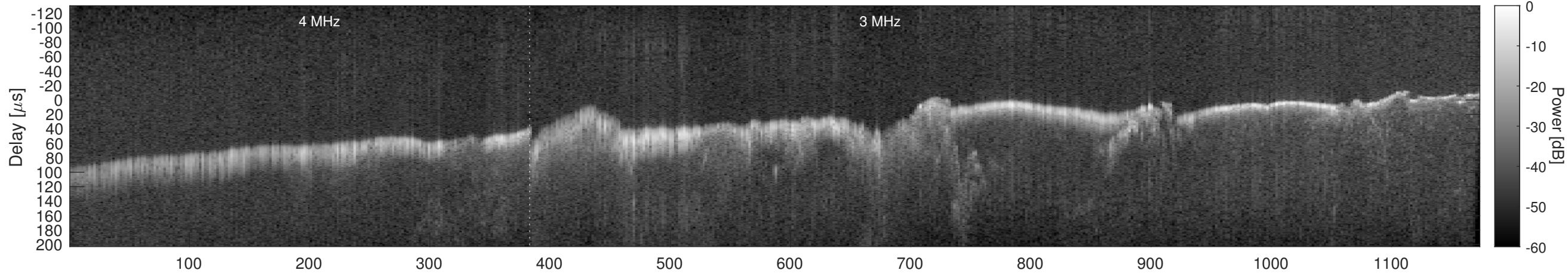
Orbit 15567, Window, Channel 2, Chapman
