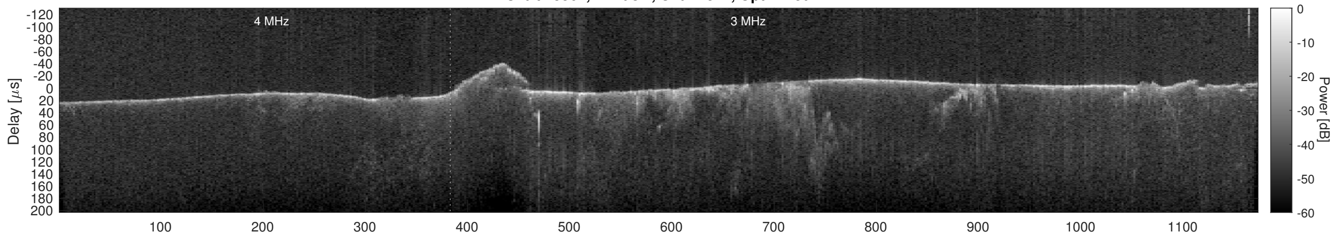
Orbit 15567, Cluttergram
