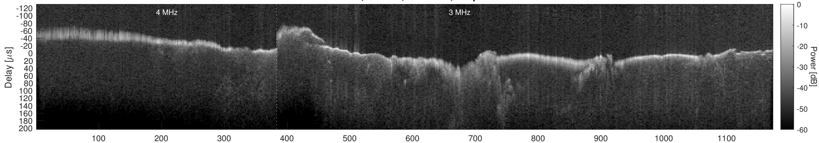
Orbit 15567, Window, Channel 2, Optimized
