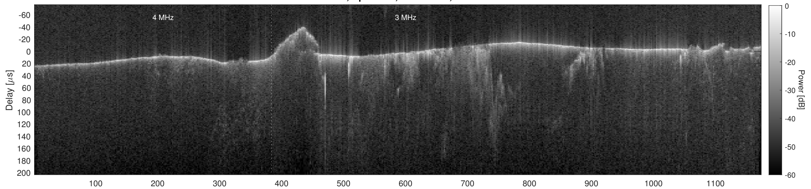
Orbit 15567, Cluttergram
