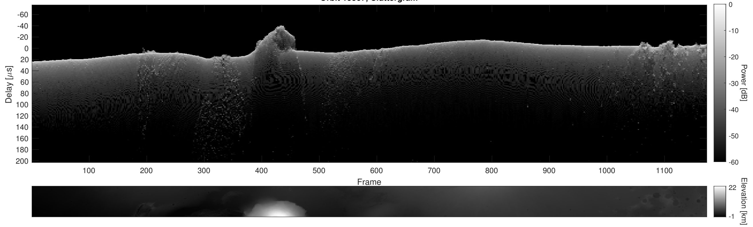
Orbit 15567, Cluttergram
