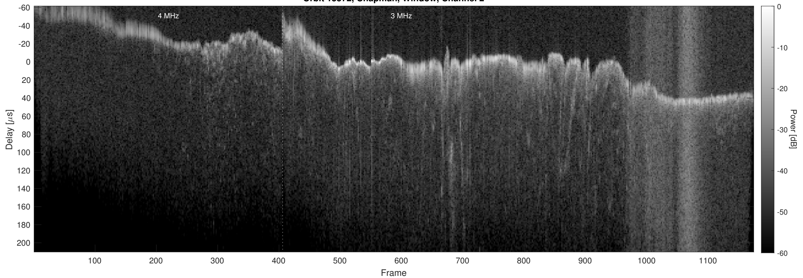
Orbit 15572, Chapman, Window, Channel 2
