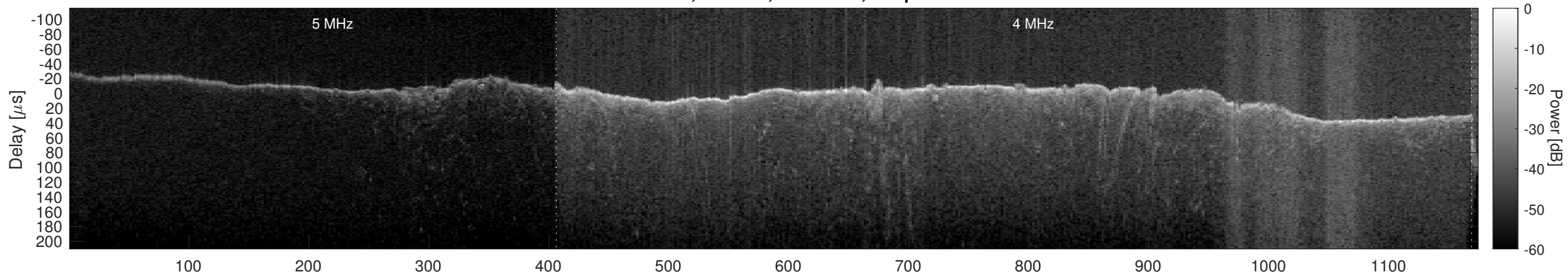
Orbit 15572, Window, Channel 1, Optimized
