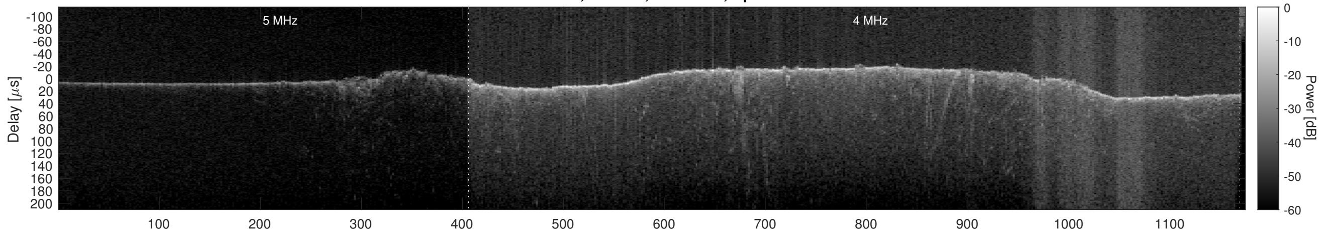
Orbit 15572, Cluttergram
