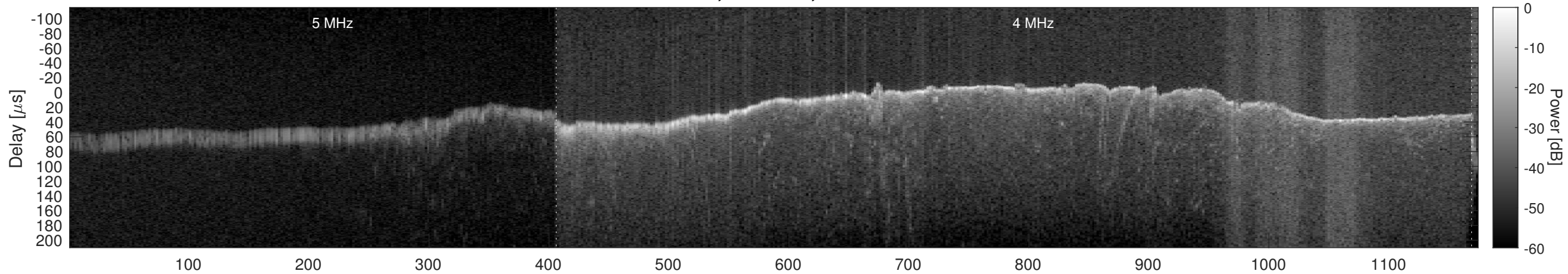
Orbit 15572, Window, Channel 1, Chapman
