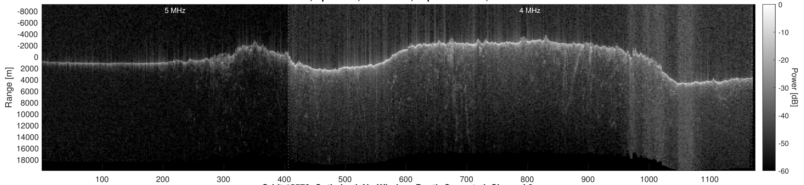
Orbit 15572, Optimized, No Window, Depth-Corrected, Channel 2
