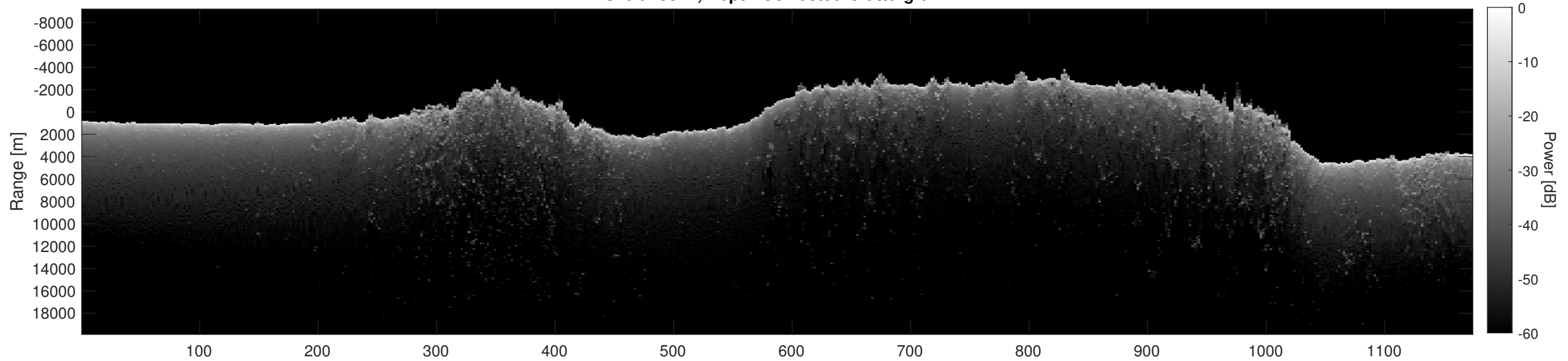
Orbit 15572, Depth-Corrected Cluttergram
