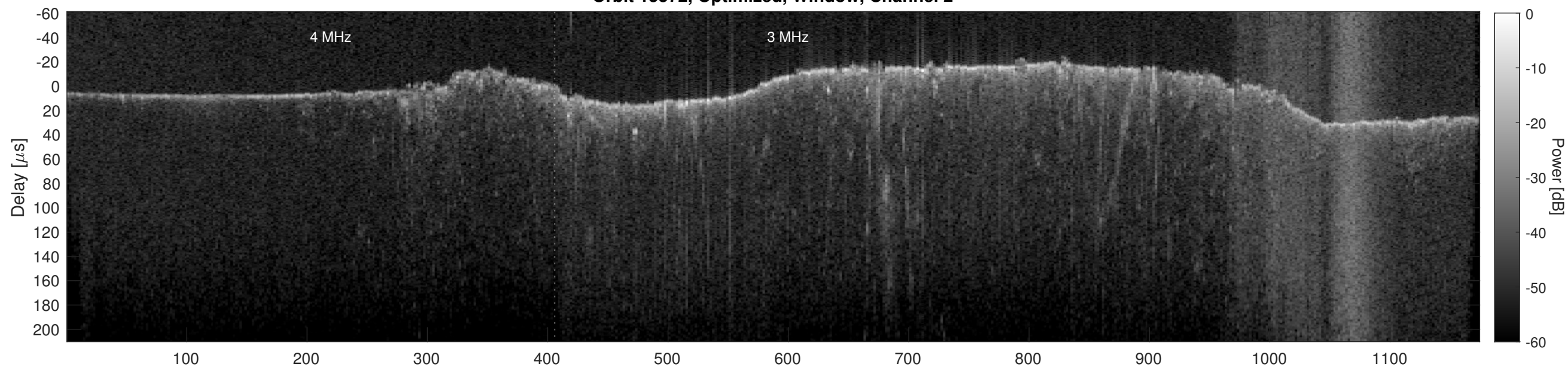
Orbit 15572, Cluttergram
