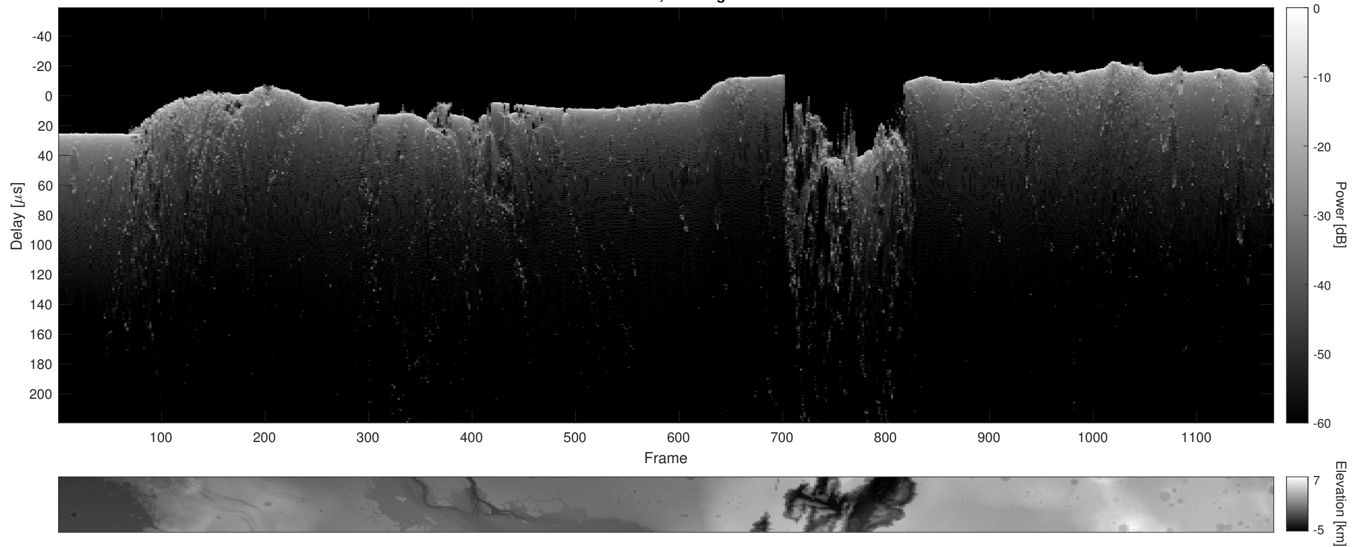
Orbit 15577, Cluttergram
