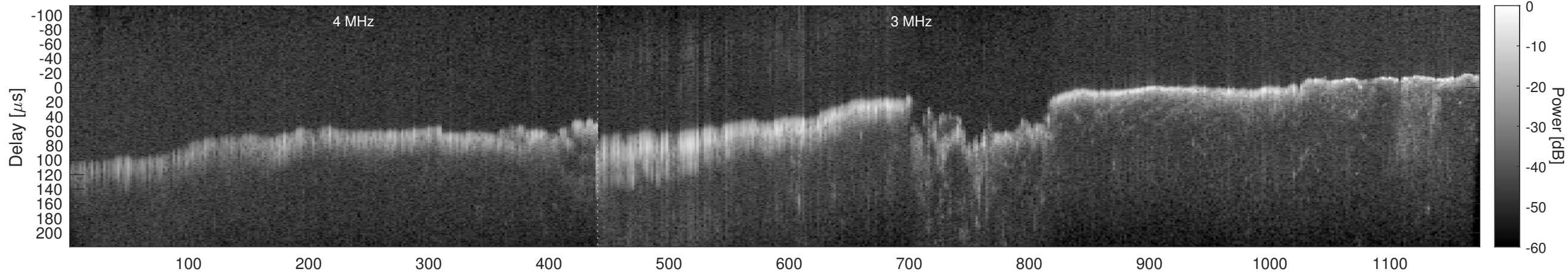
Orbit 15577, Window, Channel 2, Chapman
