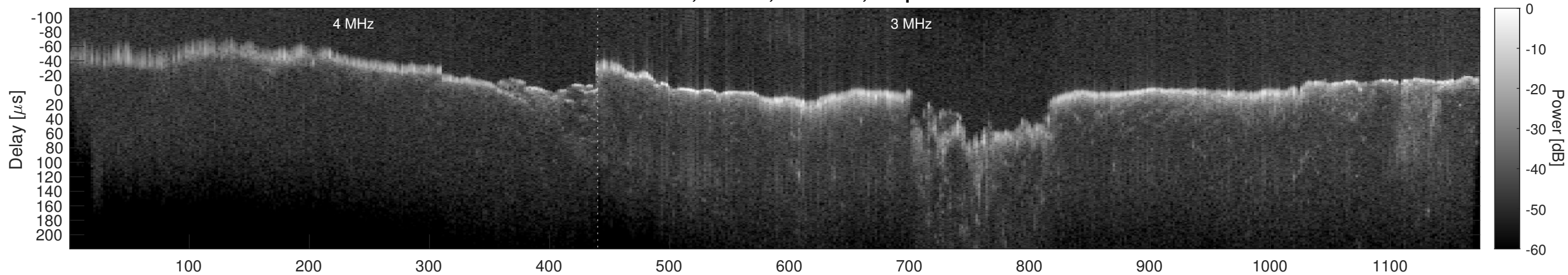
Orbit 15577, Window, Channel 2, Optimized
