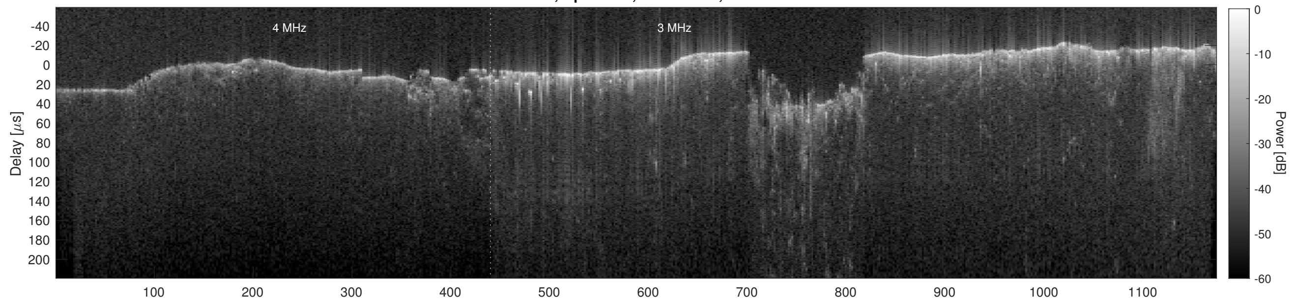
Orbit 15577, Cluttergram
