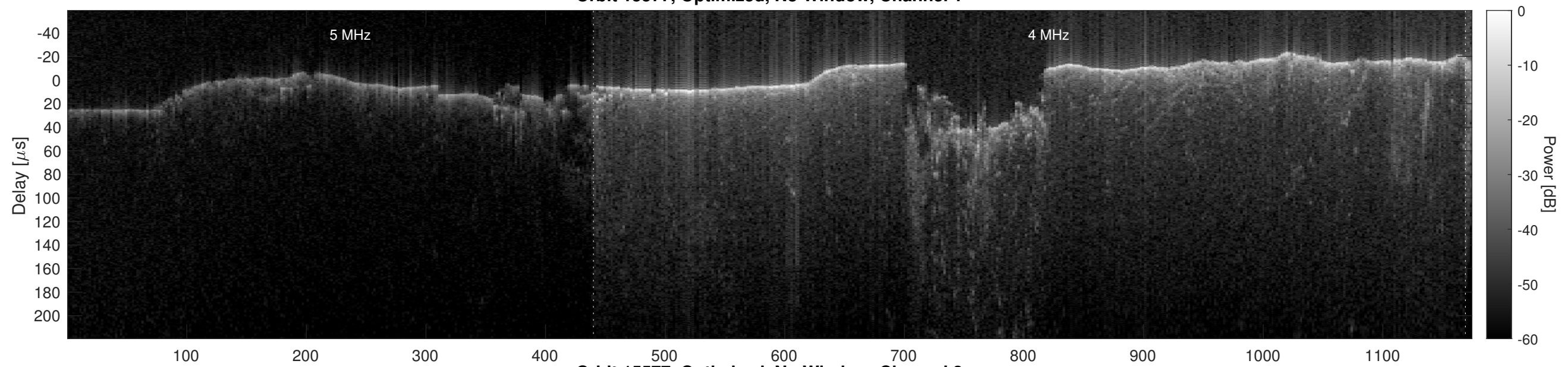
Orbit 15577, Optimized, No Window, Channel 2
