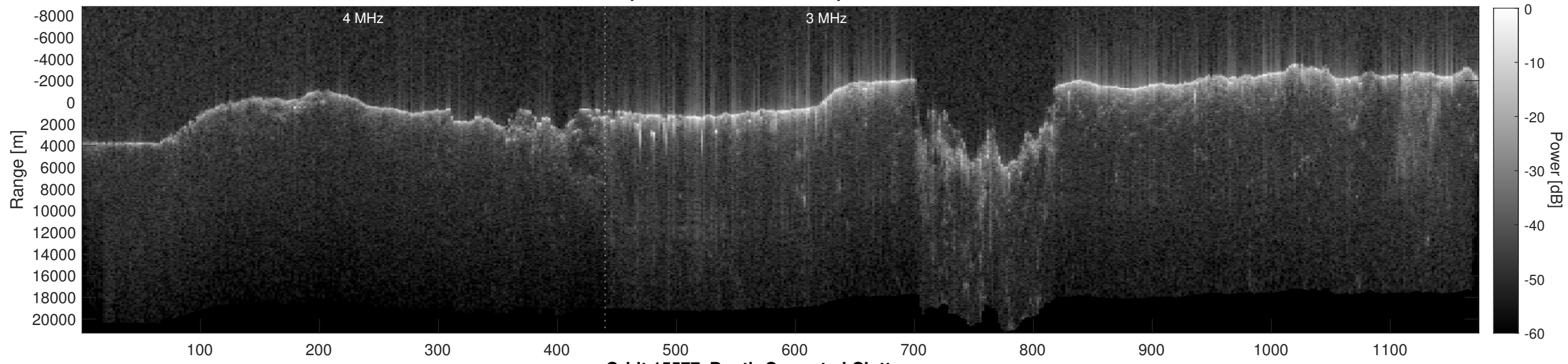
Orbit 15577, Depth-Corrected Cluttergram
