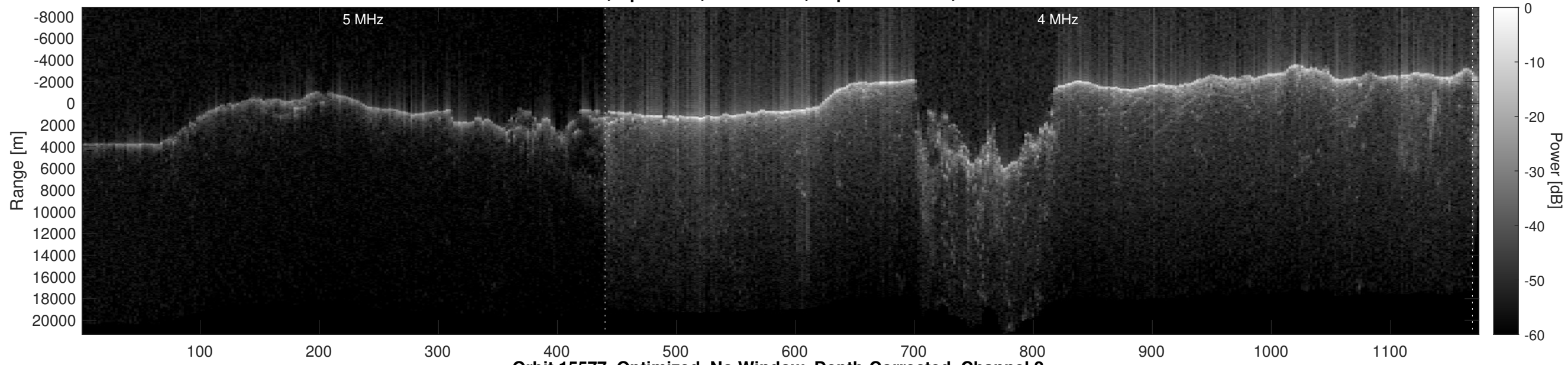
Orbit 15577, Optimized, No Window, Depth-Corrected, Channel 2
