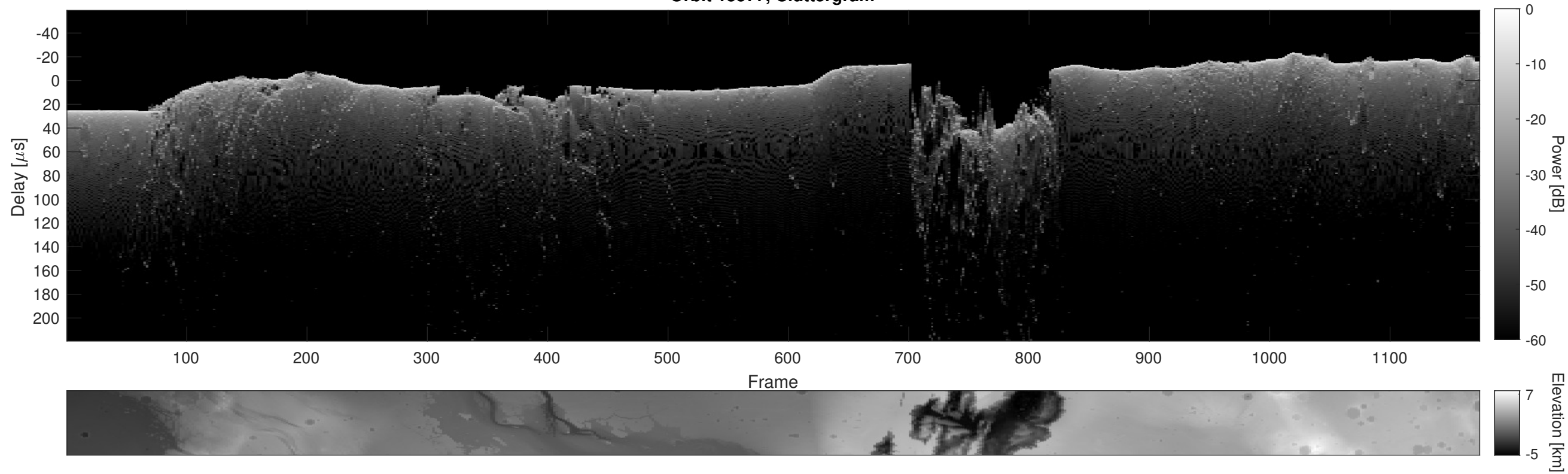
Orbit 15577, Cluttergram
