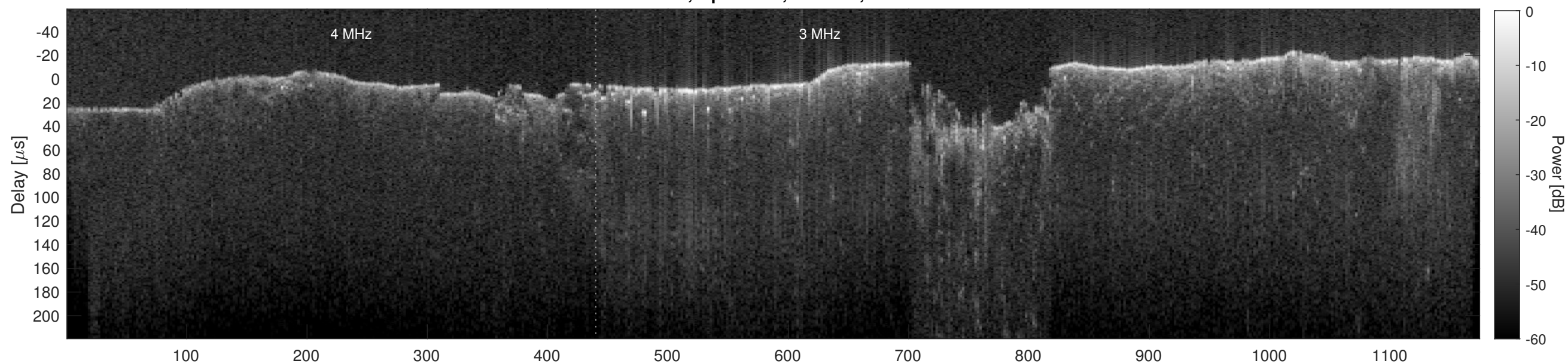
Orbit 15577, Cluttergram
