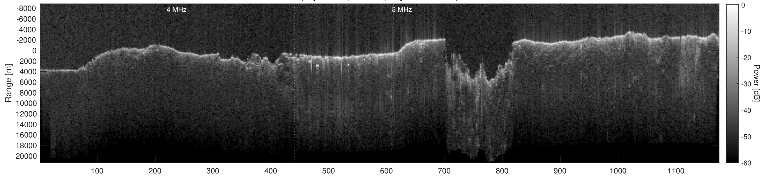
Orbit 15577, Depth-Corrected Cluttergram
