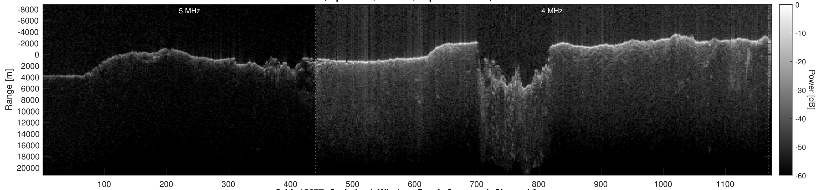
Orbit 15577, Optimized, Window, Depth-Corrected, Channel 2
