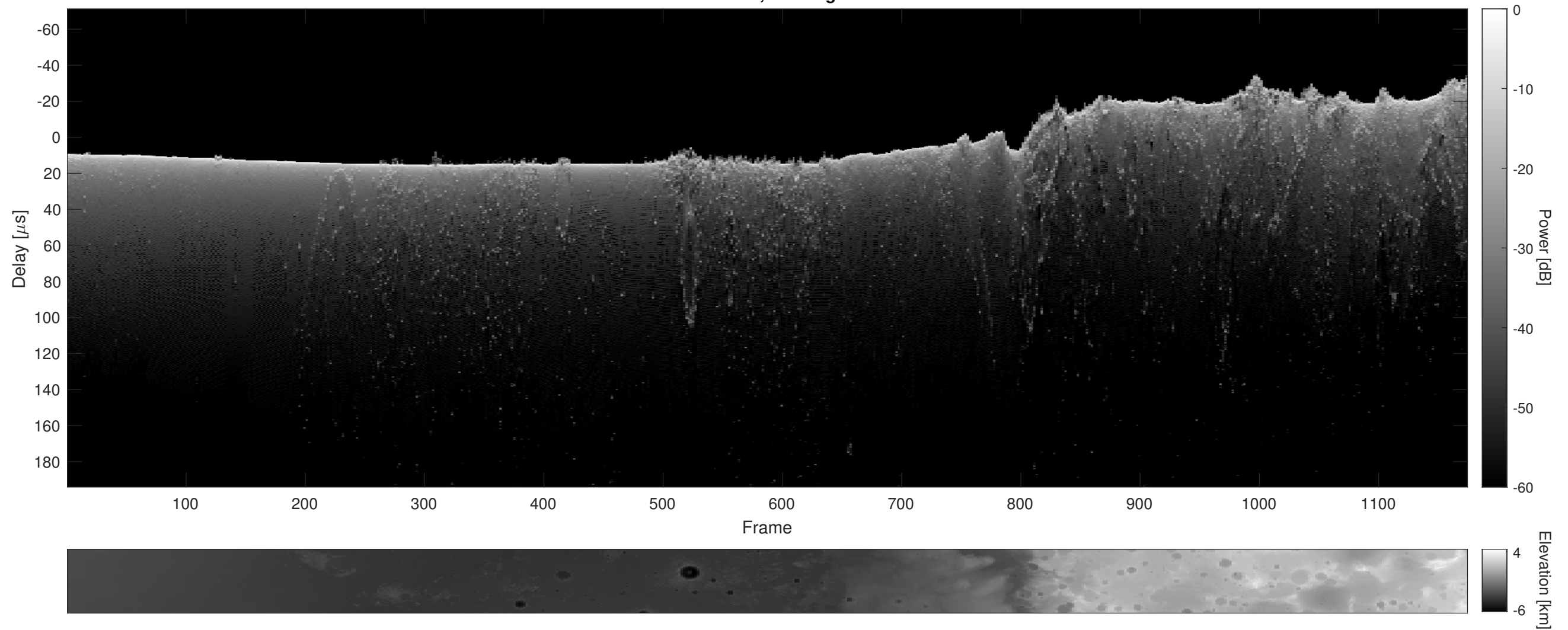
Orbit 15578, Cluttergram
