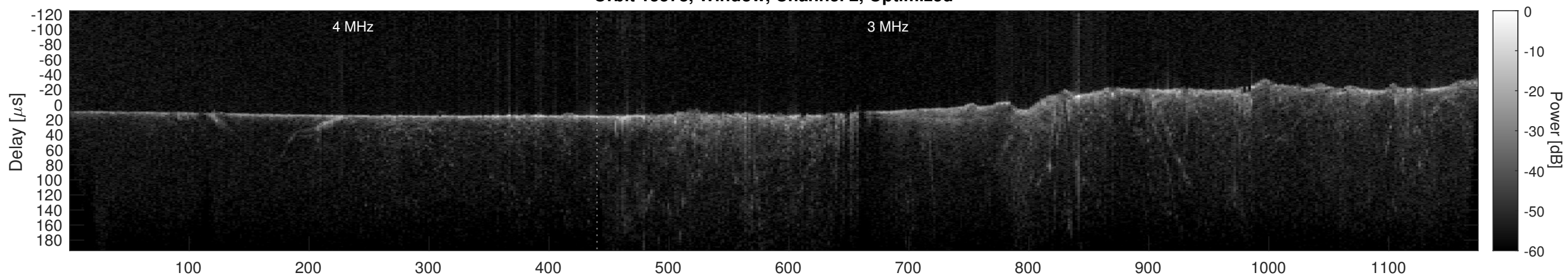
Orbit 15578, Cluttergram
