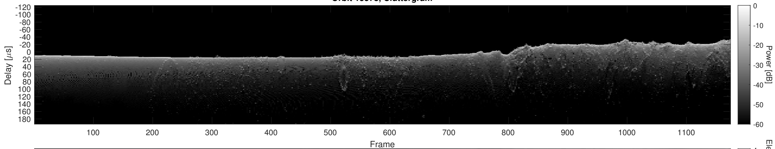
Orbit 15578, Cluttergram
