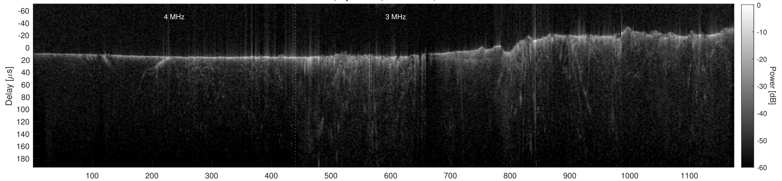
Orbit 15578, Cluttergram
