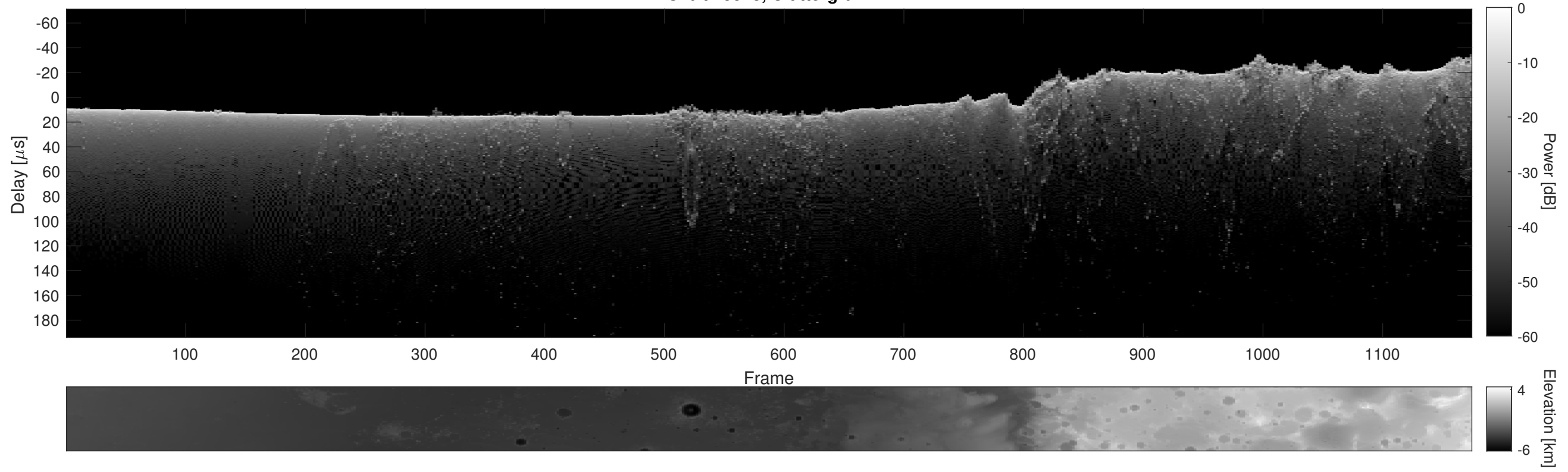
Orbit 15578, Cluttergram
