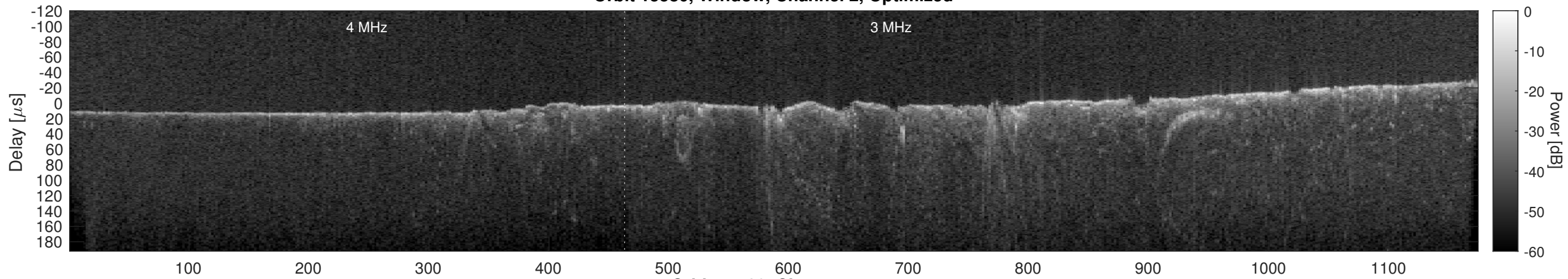
Orbit 15580, Cluttergram
