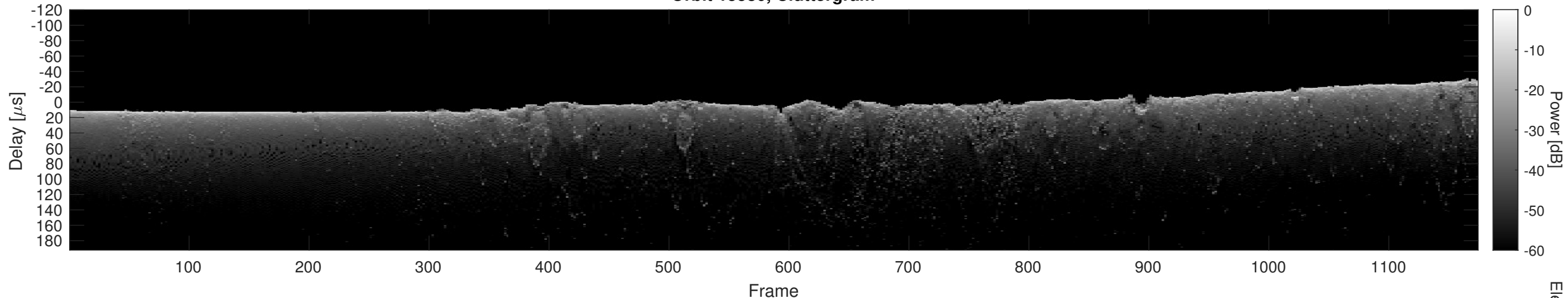
Orbit 15580, Cluttergram
