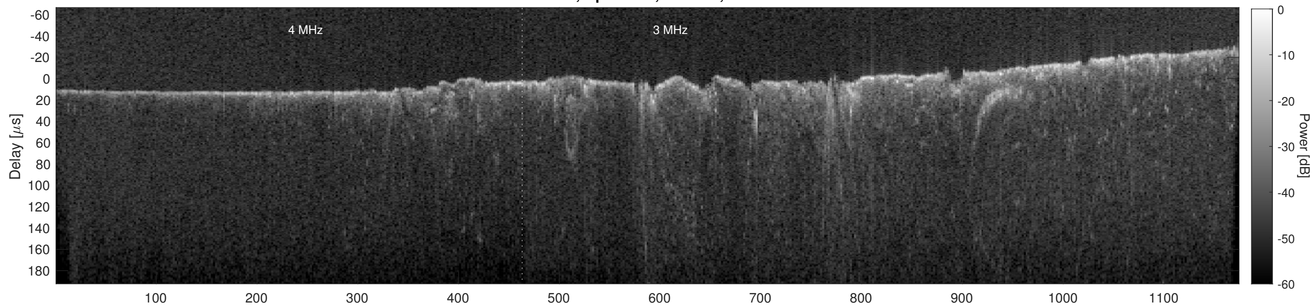
Orbit 15580, Cluttergram
