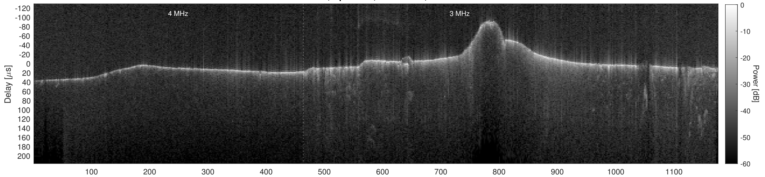
Orbit 15581, Cluttergram
