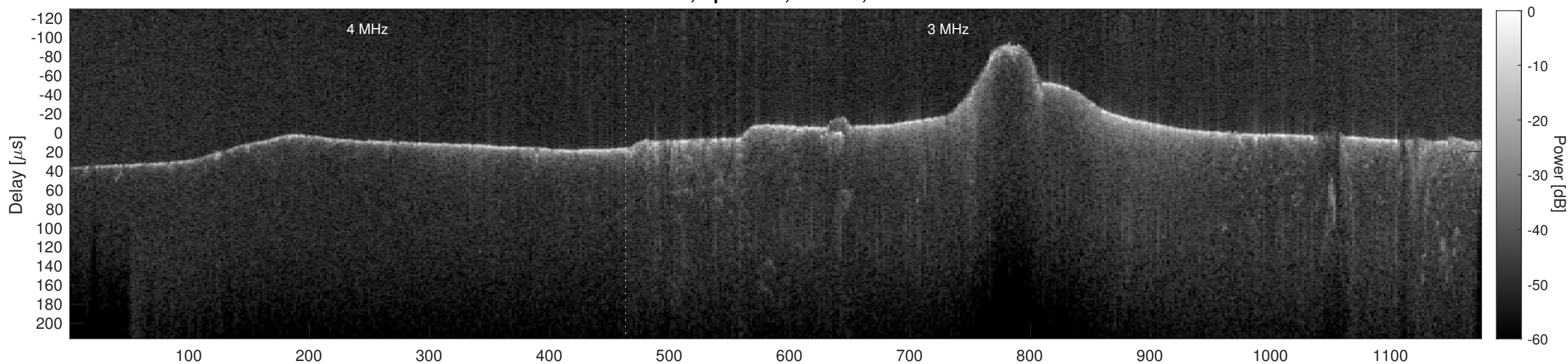
Orbit 15581, Cluttergram
