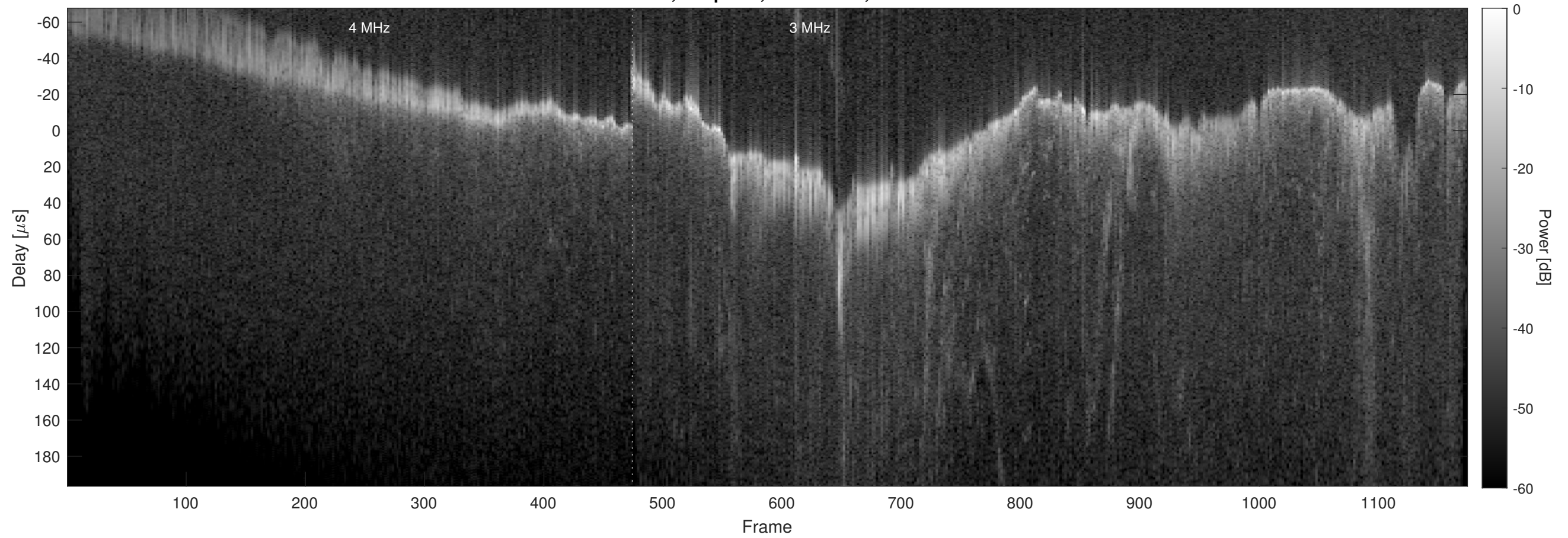
Orbit 15582, Chapman, No Window, Channel 2
