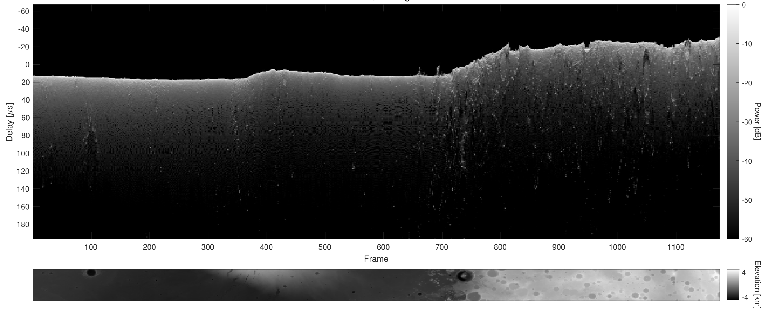
Orbit 15582, Cluttergram
