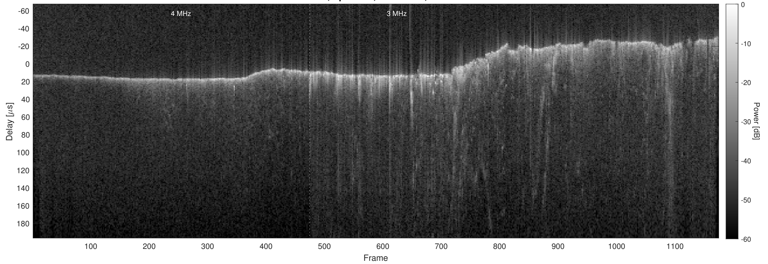
Orbit 15582, Optimized, No Window, Channel 2
