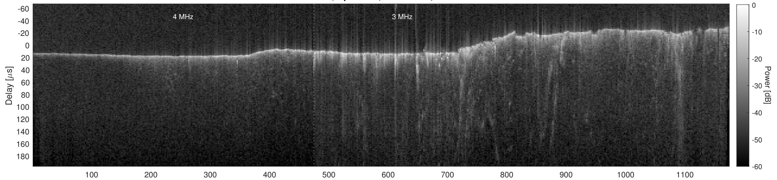
Orbit 15582, Cluttergram
