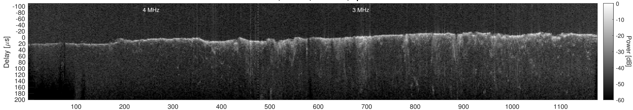
Orbit 15583, Cluttergram
