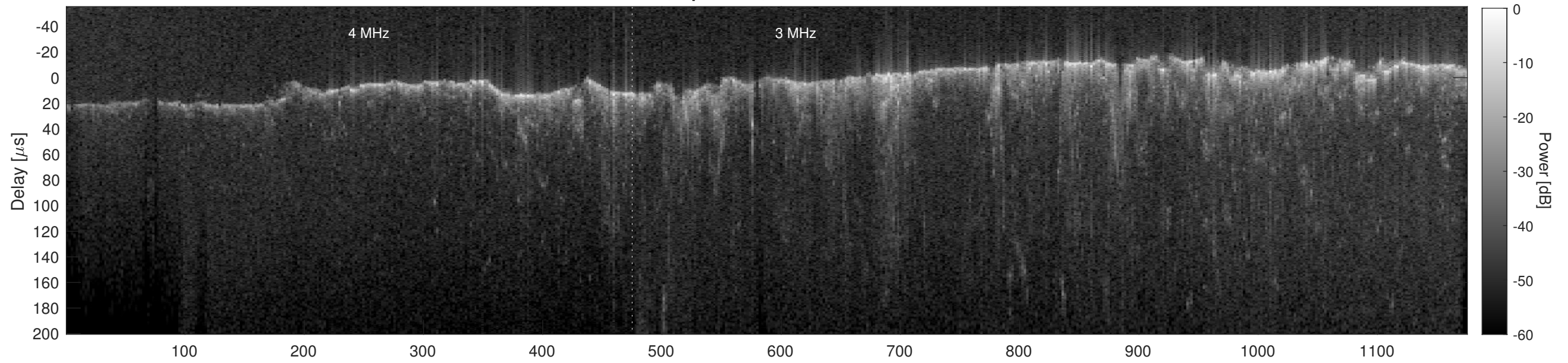
Orbit 15583, Cluttergram
