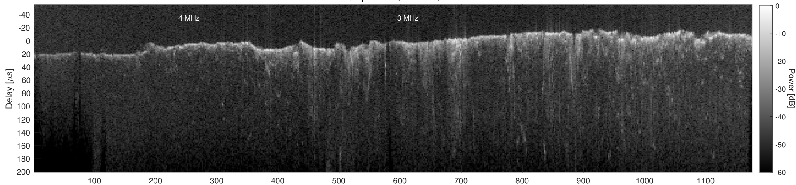
Orbit 15583, Cluttergram
