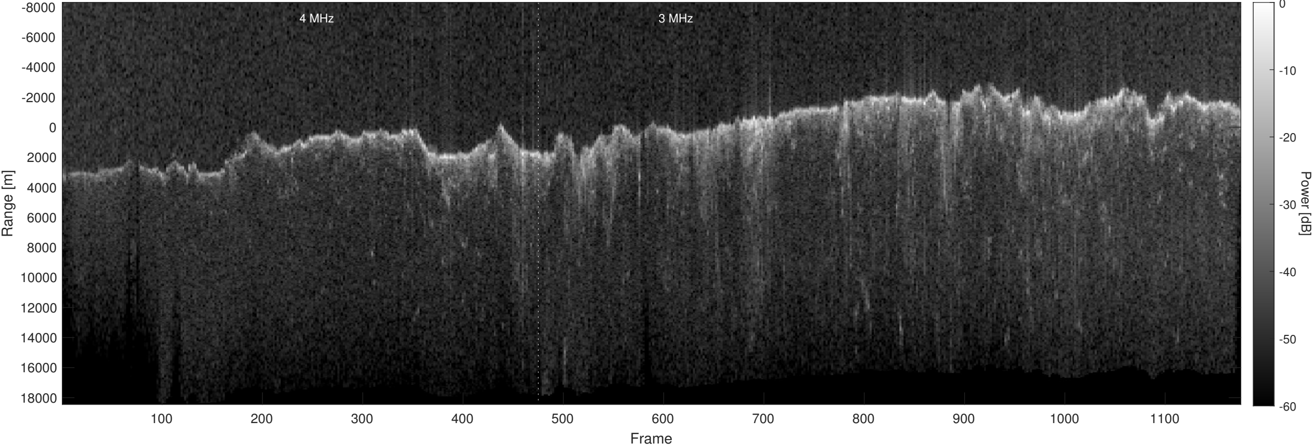
Orbit 15583, Optimized, Window, Depth-Corrected, Channel 2
