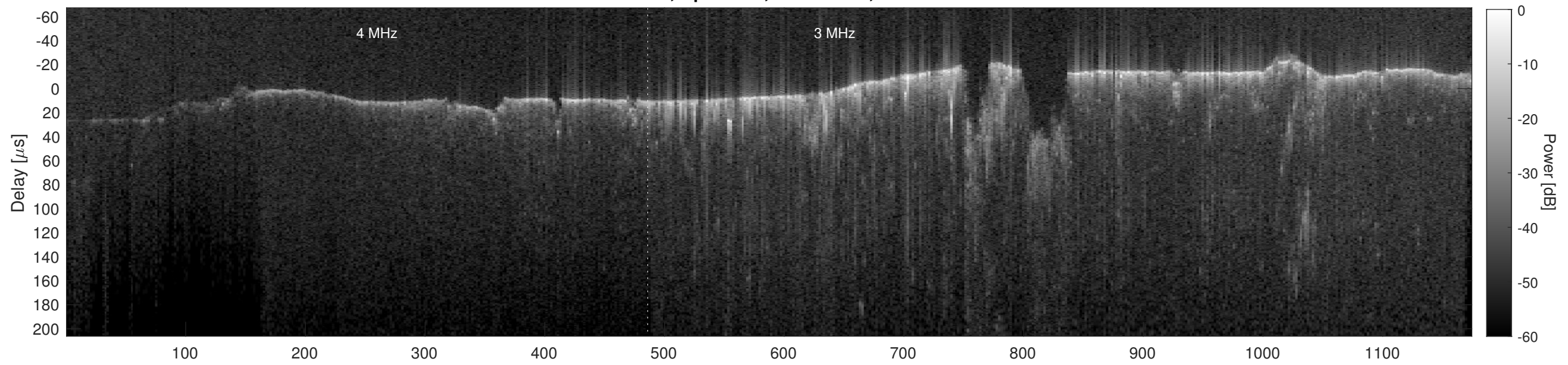
Orbit 15584, Cluttergram
