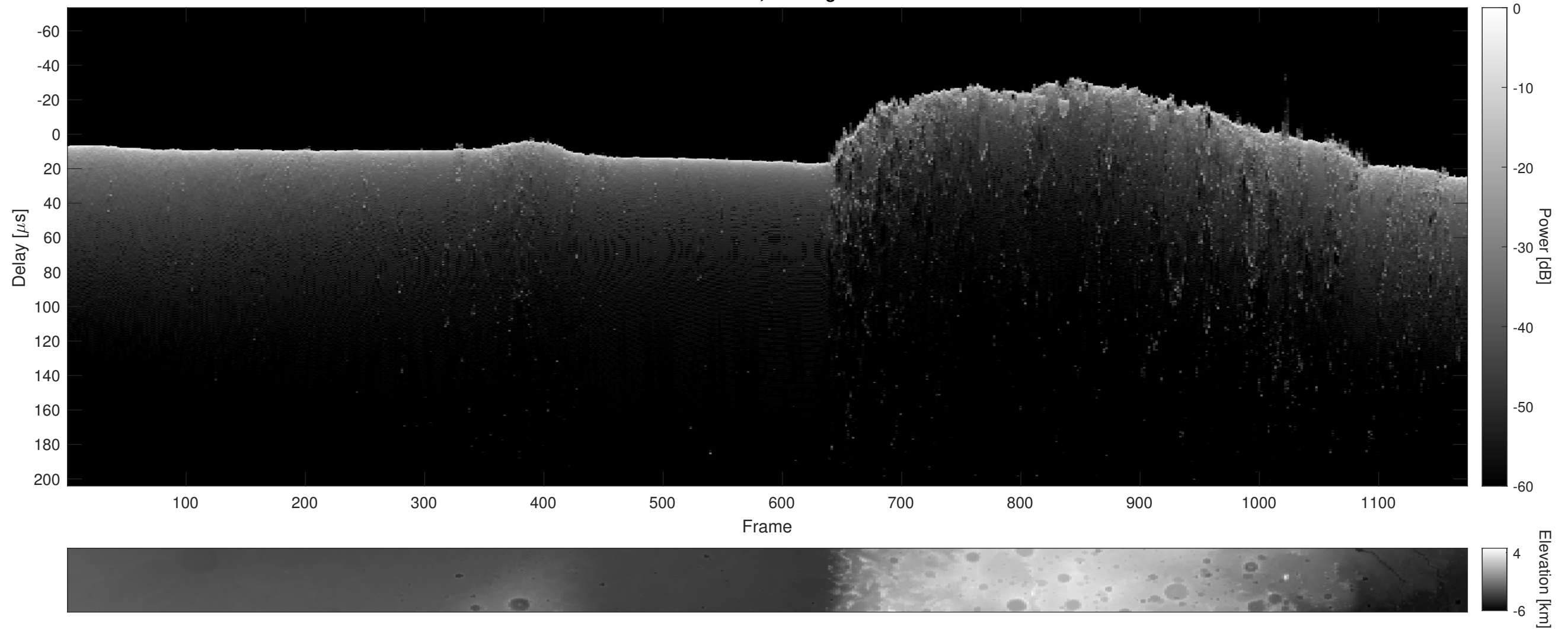
Orbit 15586, Cluttergram
