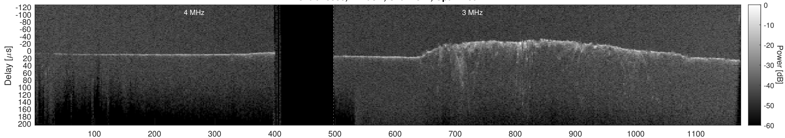
Orbit 15586, Cluttergram
